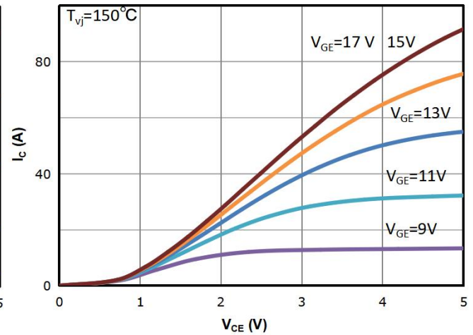
Fig 2: Output Characteristics
